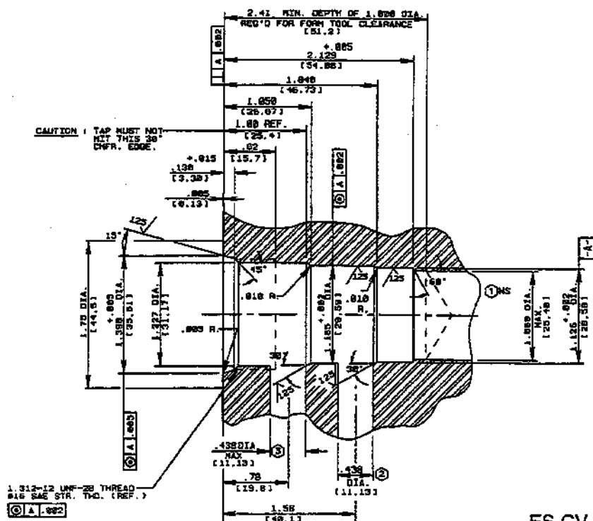
HSSCV-800-3 Form Tool
