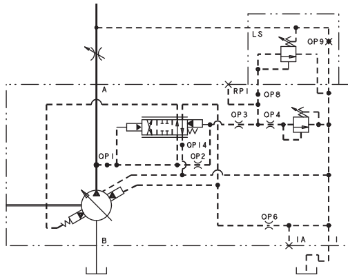
HYDRAULIC CIRCUIT
