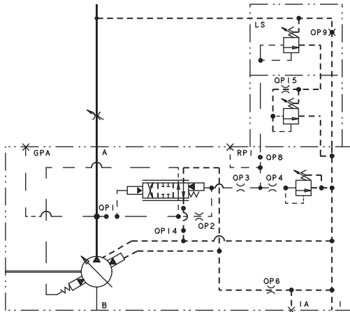
HYDRAULIC CIRCUIT
