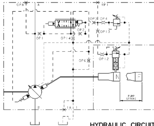
HYDRAULIC CIRCUIT
