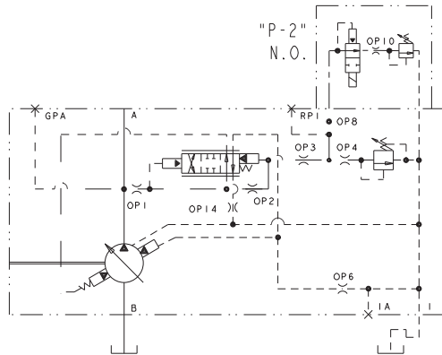
HYDRAULIC CIRCUIT
