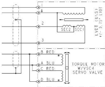
ELECTRICAL DIAGRAM
