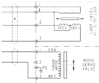
ELECTRICAL DIAGRAM
