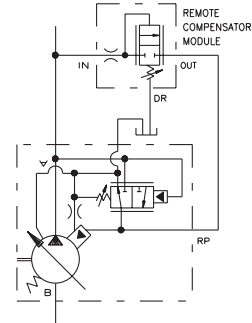
PUMP WITH REMOTE PRESSURE CONTROL
