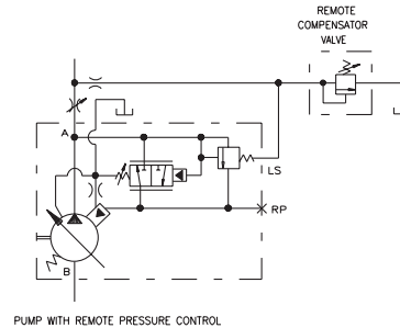
PUMP WITH REMOTE PRESSURE CONTROL
