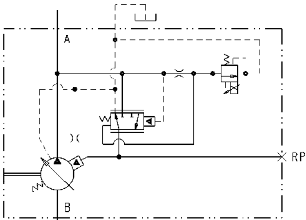
HYDRAULIC CIRCUIT PUMP WITH P-B (N.C.) CONTROL
