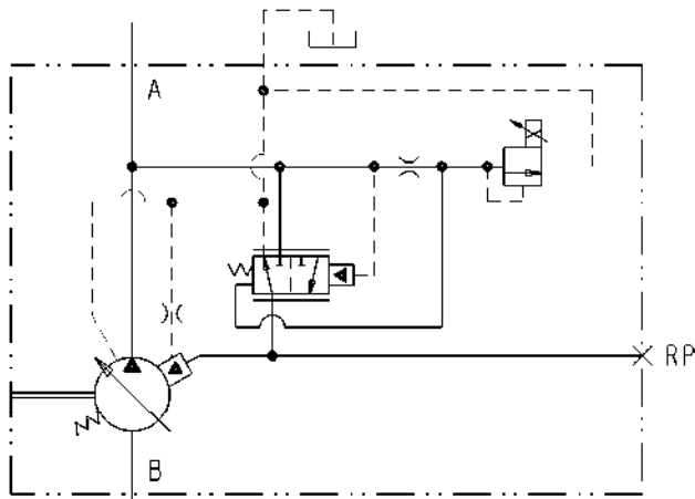
HYDRAULIC CIRCUIT PUMP WITH P-A (N.O.) CONTROL
