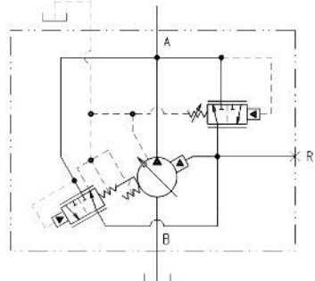
HYDRAULIC CIRCUIT
