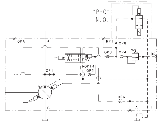
HYDRAULIC CIRCUIT
