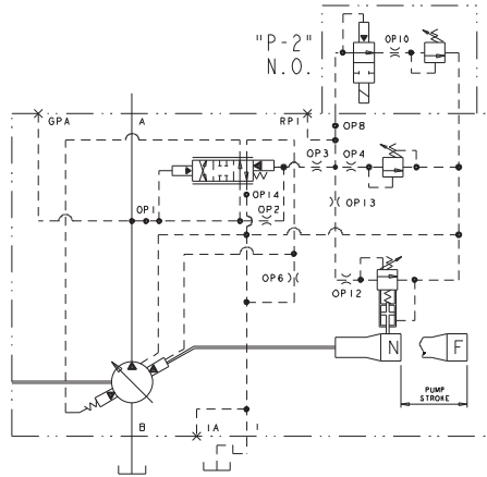
HYDRAULIC CIRCUIT
