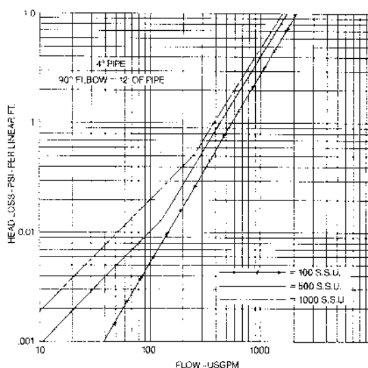
4" PIPE
