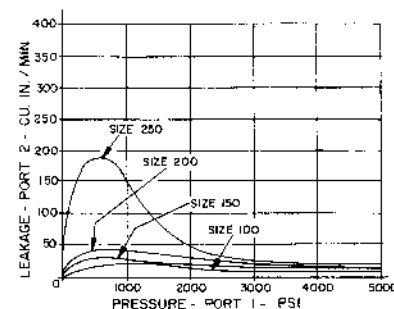
Average Leakage (Port 1 to 2) vs Line Pressure Typical for 500 SSU fluid
