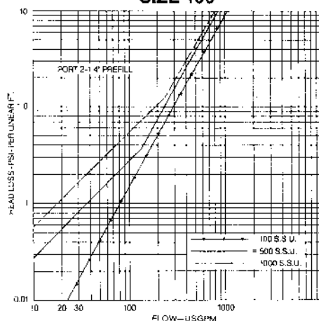
Pressure Drop vs Flow, Port 2 to Port 1
