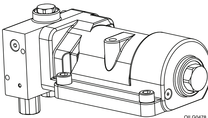
Figure 1. Typical Oilgear Type “P-1NN” Single Pressure Compensator Control for PVG-150 Pumps
