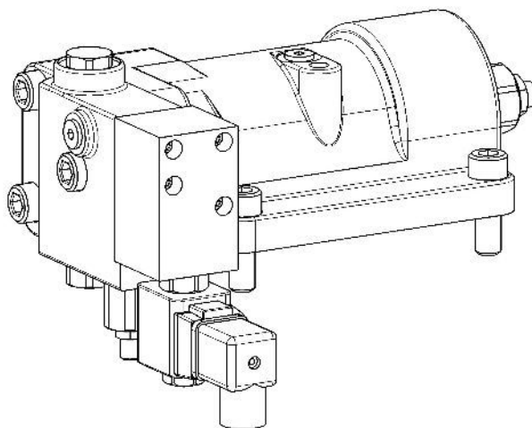
Figure 1. Typical Oilgear Type "P-C & P-K" Single Pressure - Soft Start Control for PVG-150 Pumps
