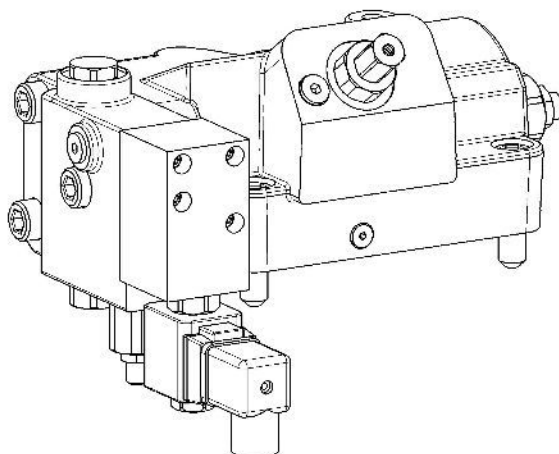
Figure 1. Typical Oilgear Type "P-CNN/H & P-KNN/H" Single Pressure - Soft Start with Horsepower Limiter, Control for "PVG" 150 Pumps
