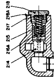
SECTION E-E
