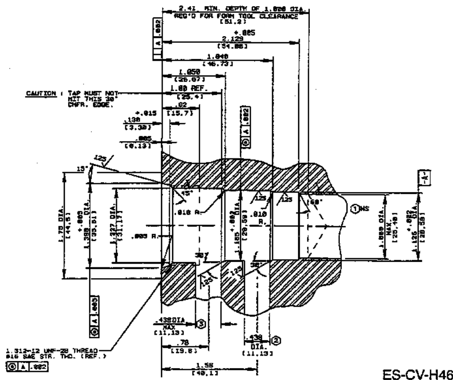
HSSCV-800-3 Form Tool
