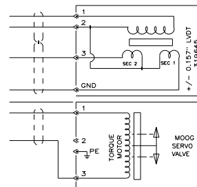
ELECTRICAL CIRCUIT
