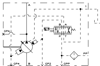
HYDRAULIC CIRCUIT
