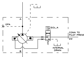
HYDRAULIC CIRCUIT
