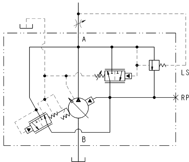
HYDRAULIC CIRCUIT
