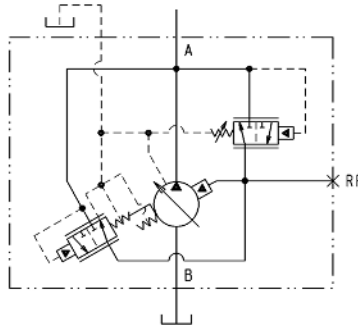
HYDRAULIC CIRCUIT
