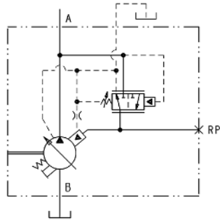
HYDRAULIC CIRCUIT PUMP WITH P-H CONTROL
