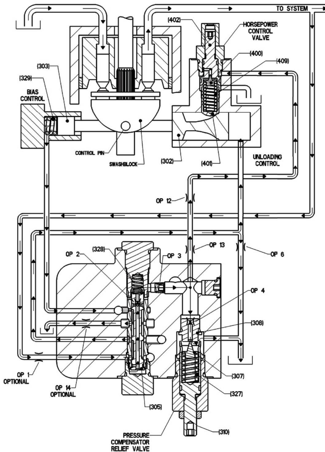
Figure 5. Compensating Pressure - Unloading
