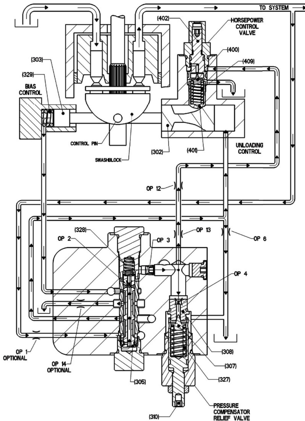
Figure 6. Compensating Pressure (Unloading) - Horsepower Limiter Active
